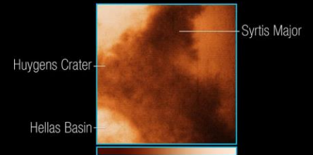
NIRCam brightness at 2.1 microns
