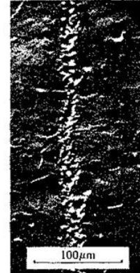
Arc track in the DITE tokamak. McCracken et al. Nucl. Fusion (1978)
