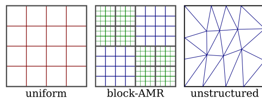
Figure 25. Schematic illustration of three types of numerical grids in 2D. Uniform grids are the simplest to work with. Adaptive mesh refinement (AMR) allows for a varying resolution in the domain, and unstructured grids are the most flexible.
