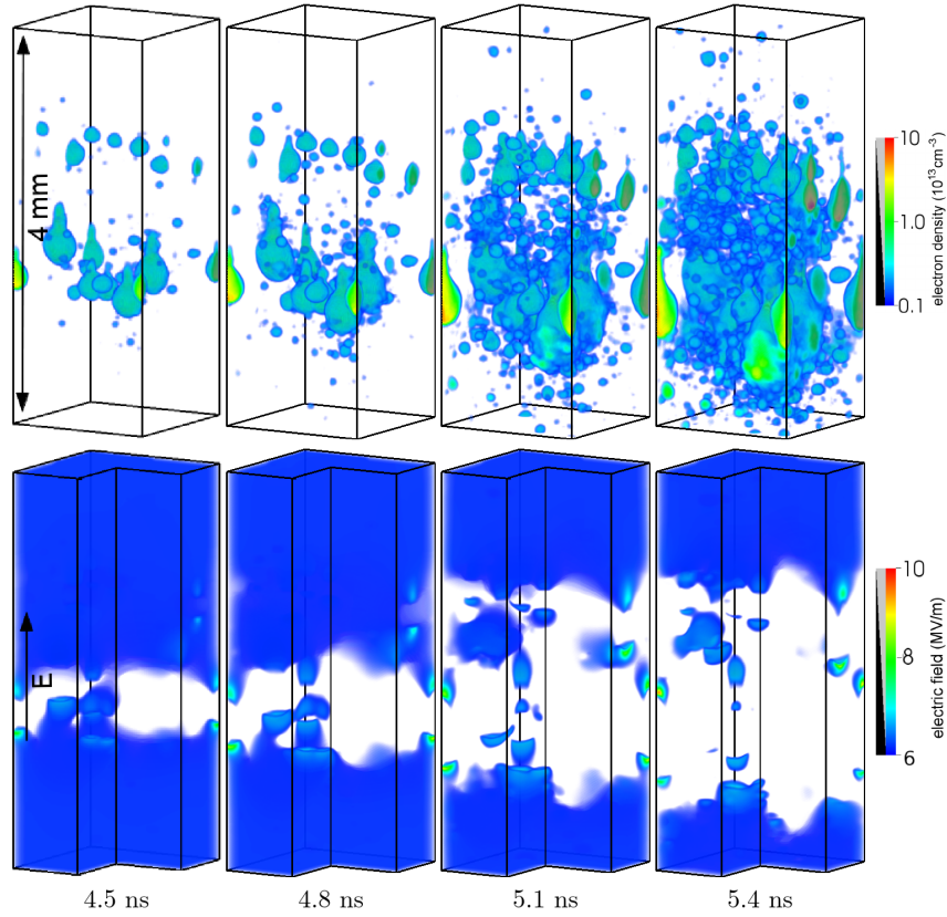
Figure 8. Simulation of discharge inception in atmospheric air in a field of twice the breakdown value, taken from [37]. Shown are the electron density (top) and electric field (bottom). Initially, a layer of O_2^- ions with a density of 10^4 \text{ cm}^{-3} was present. Electrons detach from these ions and form multiple overlapping avalanches.
