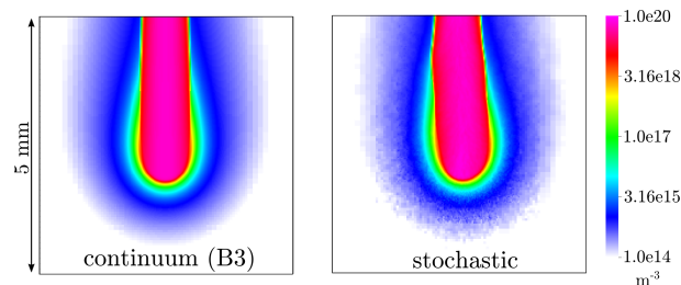
Figure 12. Cross sections through 3D simulations of positive streamers in air, showing the electron density on a logarithmic scale. Two photo-ionization models are used: a continuum approximation [61] (left) and a stochastic (Monte Carlo) model with discrete single photons (right). Due to the large number of ionizing photons in air, individual electron avalanches cannot be distinguished, and the continuum approximation works well. Figure adapted from [62].
