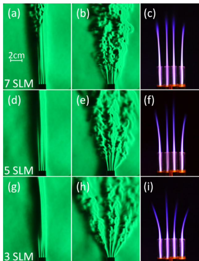
Figure 22. Image from [166] showing a helium jet array operating at gas flow rates of 7, 5 or 3 SLM in the upper (a-c), middle (d-f) and lower (g-i) row. The left column (a, d, g) shows Schlieren images of the gas flow without applied electric field, and the middle column (b, e, h) with the plasma voltage switched on. The right column (c, f, i) shows camera images of the plasma plume trajectory for the case when the voltage is on.
