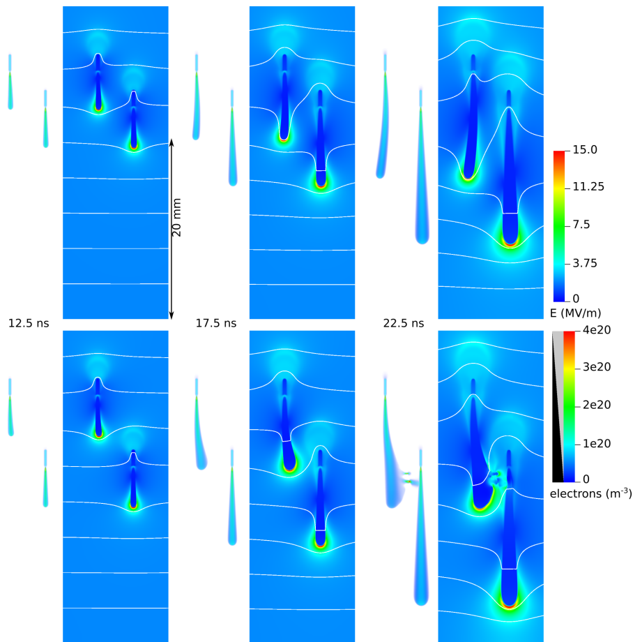
Figure 19. 3D Plasma fluid simulations interacting positive streamers in atmospheric air. The streamers start from two ionized seeds, which have a vertical offset of 4 mm (top row) or 8 mm (bottom row), which leads to repulsion and attraction, respectively. The images show the electron density (volume rendering) and cross sections of the electric field with equipotential lines spaced by 4 kV. Picture taken from [22].
