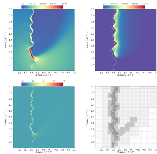
Figure 26. 2D simulation with adaptive mesh refinement of a positive streamer propagating over a rough dielectric surface. Figure taken from [265]
