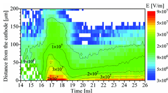
Figure 28. Electric-field strength distribution in repetitive Trichel pulse in atmospheric-pressure air measured with cross-correlation spectroscopy using the nitrogen line ratio method. Image from [344].
