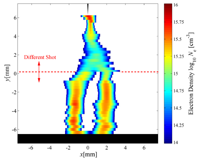
Figure 29. Two dimensional electron density distribution acquired by measuring refractive index variations. Image from [88].
