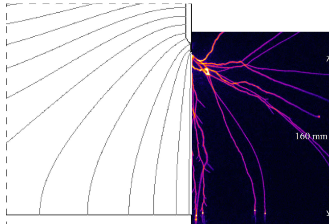
Figure 16. Comparison of calculated background electric field lines with streamer paths in 200 mbar nitrogen with 0.2 % oxygen admixture in a 16 cm point plane-gap with a +11.0 kV pulse. Image adapted from [25].
