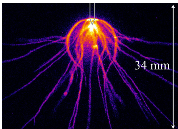
Figure 1. A long exposure, false colour, image of a peculiar streamer discharge caused by a complex voltage pulse. Image taken from [1].
