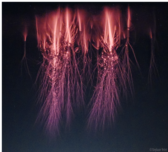
Figure 23. Colour image of a sprite discharge in the upper atmosphere. Image is a frame from a video (Sony A7s - Nikkor 105mm/1,4@1,4 - Atomos Shogun - 1/25s - 64000 ISO). Location & Time: Peninsula Orbetello, Italy - 10 September 2019 2h UTC. Image courtesy of Stéphane Vetter and reproduced with permission.
