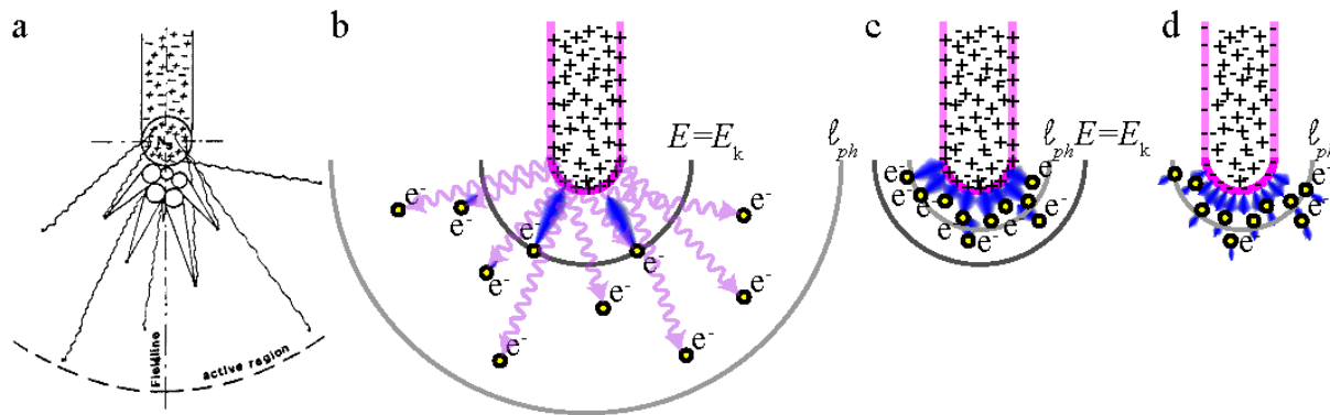
Figure 11. Schematic depictions of streamer propagation. a) Illustration of positive streamer propagation in air based on the original concept of Raether [59], published in English by Loeb and Meek [60]. Picture taken from [32]. Panels b-d) show an updated scheme for b) positive streamers with few photons with a long mean free path, c) positive streamers in air and d) negative streamers in air. Avalanches start from a yellow electron and are indicated in blue, \ell_{\text{photo}} indicates the photo-ionization range and E = E_k indicates the active region. Note also that panel a) shows a net positive charge in a spherical head region, while panels b-d) show have surfaces charges around the streamer head and along the lateral channel.
