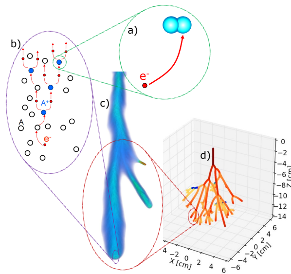
Figure 4. The multiple spatial scales in streamer discharges: a) collision of an electron with an atom or molecule, b) multiple electrons accelerate in a local electric field, collide with neutral gas molecules and form an ionization avalanche, c) a branching streamer discharge with field enhancement at the tips, d) a discharge tree with multiple streamer branches. Panel d is reproduced from a figure in [24].
