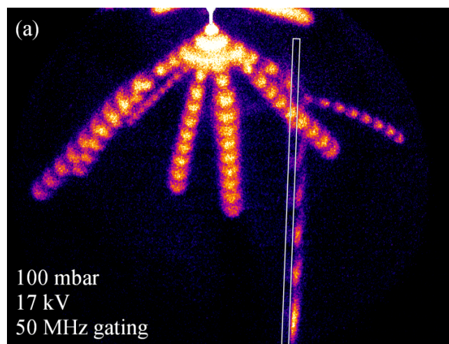
Figure 27. Stroboscopic ICCD image of a streamer discharge in artificial air in the vicinity of a dielectric rod. Image from [134].
