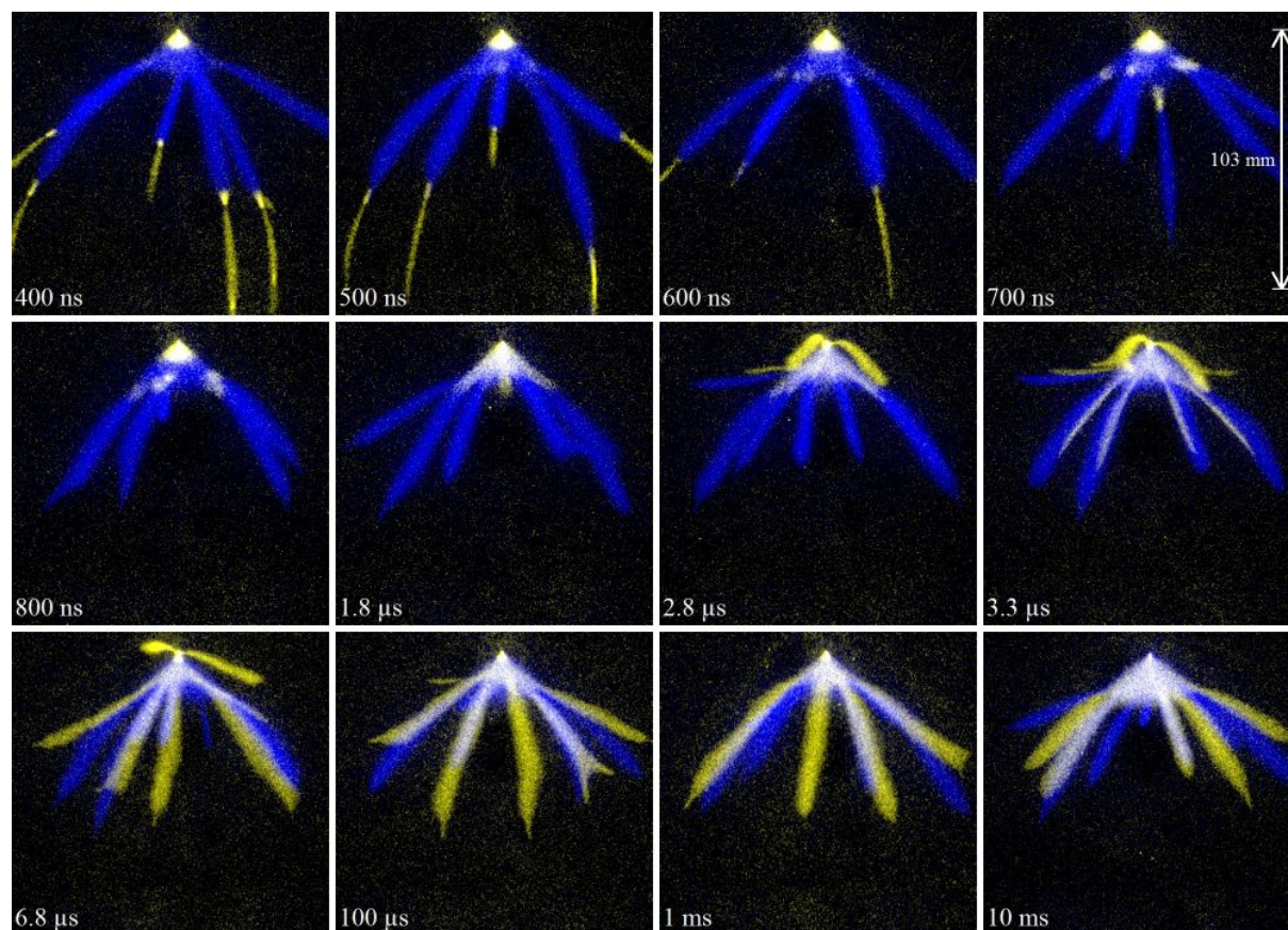
Figure 18. Superimposed discharge-pair images for varying pulse-to-pulse delays (as indicated in the images). Images taken in 133 mbar artificial air with pulses of 13.6 kV amplitude and 200 ns pulse length in a 103 mm point plane gap. A blue color indicates intensity recorded during the first pulse, yellow during the second pulse and white during both pulses. Image from [110].
