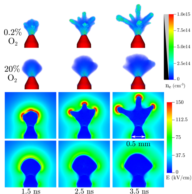
Figure 10. Particle-in-cell simulation of discharge inception around a needle electrode. Two gases are used: \text{N}_2 with 20% and 0.2% \text{O}_2 , both at 1 bar. The electron density (top) and a cross section of the electric field (bottom) are shown. Figure adapted from [58].
