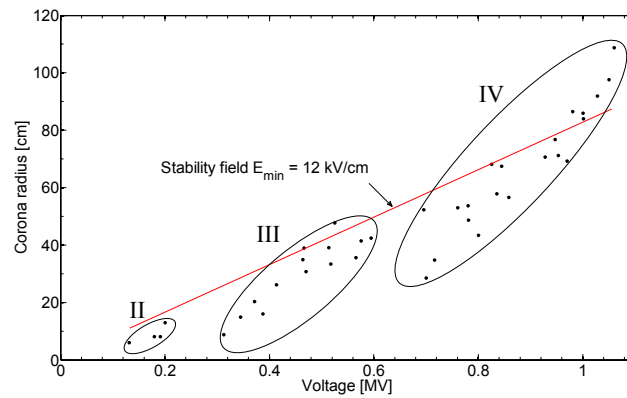
Figure 15. Radius of the negative corona as a function of voltage in a gap of 127 cm length in ambient air, obtained from 39 discharges. The voltage increases to 1 MV within 1.2 \mu\text{s} , so the voltage axis corresponds roughly to a time axis. The growth of this discharge in ICCD images is shown in the lower panel of figure 7. The so-called stability field of 12 \text{ kV cm}^{-1} is indicated with a red line. The second, third and fourth streamer bursts are indicated with II, III, IV and encircled by ellipsoids. Image from [28].
