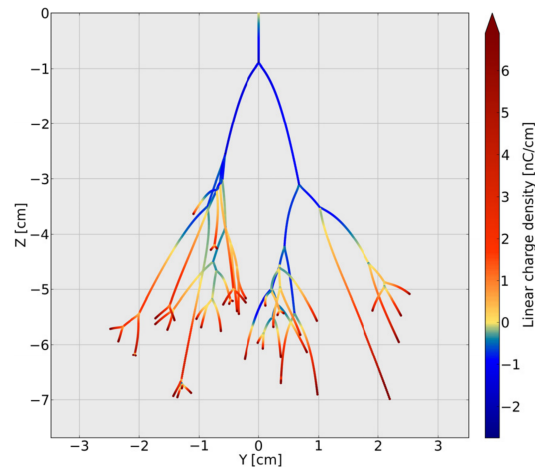
Figure 24. Charge distribution in a streamer simulation using a tree model. Picture taken from [24]. The color scale is truncated and does not show the charge density at the streamer tips, as they would dominate the plot.
