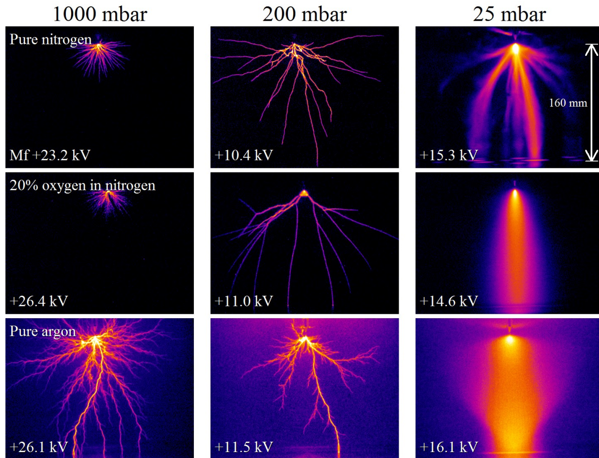
Figure 6. Overview of positive streamer discharges produced in three different gas mixtures (rows), at 1000, 200 and 25 mbar (columns). All measurements have a long exposure time and therefore show the whole discharge, including transition to glow for 25 mbar. Image adapted from [26].
