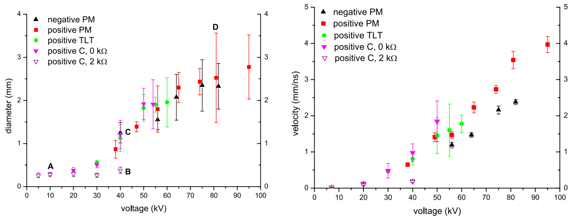
Figure 13. Diameter (left) and velocity (right) of streamers as a function of applied voltage and polarity, reproduced from [67]. The different voltage sources and their voltage rise times are 15 ns for PM, 25 ns for TLT, 30 ns for C with 0 k \Omega , and 150 ns for C with 2 k \Omega .
