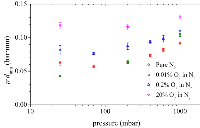
Figure 14. Scaling of the reduced minimal diameter ( p \cdot d_{\min} ) with pressure ( p ) for the four different nitrogen oxygen mixtures. Image from [26].
