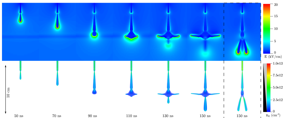
Figure 21. Simulated time evolution of a streamer discharge propagating in pure nitrogen and interacting with a 10^9 \text{ cm}^{-3} preionized trail. Top row: cross sections of the electric field, bottom row: volume rendering of the electron density. For the rightmost figures, the viewpoint has been rotated by 90^\circ , revealing that the downwards streamer has branched. Image from [107].
