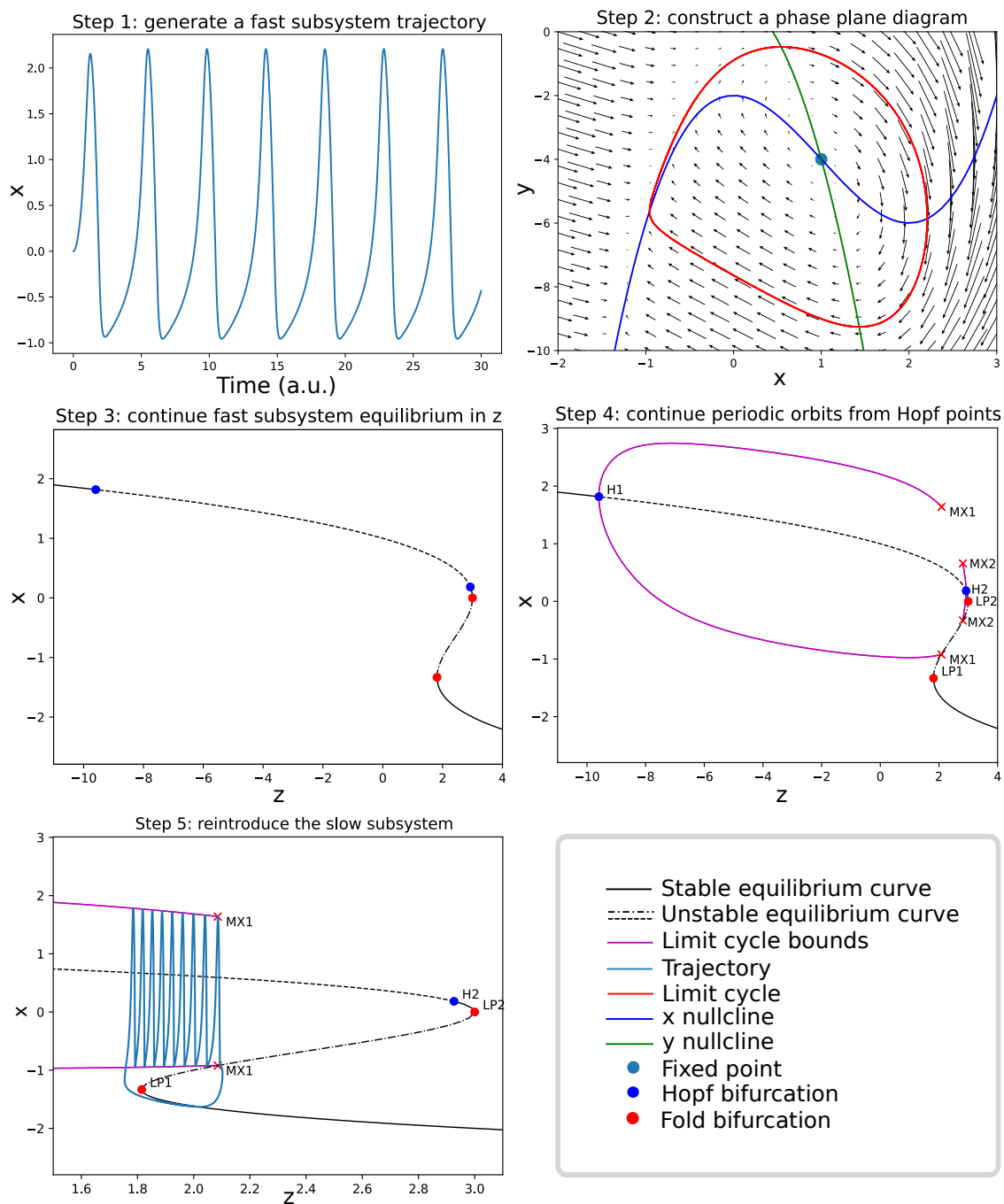
Figure 2: Investigating the cause of bursting in the Hindmarsh Rose model. Dark blue dots, labelled ‘H’, indicate a Hopf bifurcation. Red dots, labelled ‘LP’, indicate a limit point, or fold, bifurcation. Red crosses, labelled ‘MX’, indicate the end of continuation, here demarcating a homoclinic bifurcation. A solid black line represents a stable equilibrium location; a dashed black line indicates an unstable equilibrium location; a purple line represents the maximum and minimum values of a limit cycle. Trajectories are shown as light blue lines.
