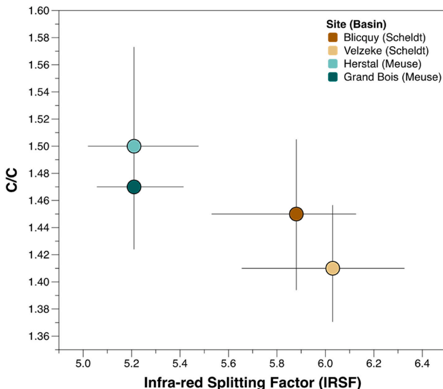
Fig. 3. Median C/C to IRSF values of the studied sites. The error bars indicate the 1st and the 3rd quartiles.
