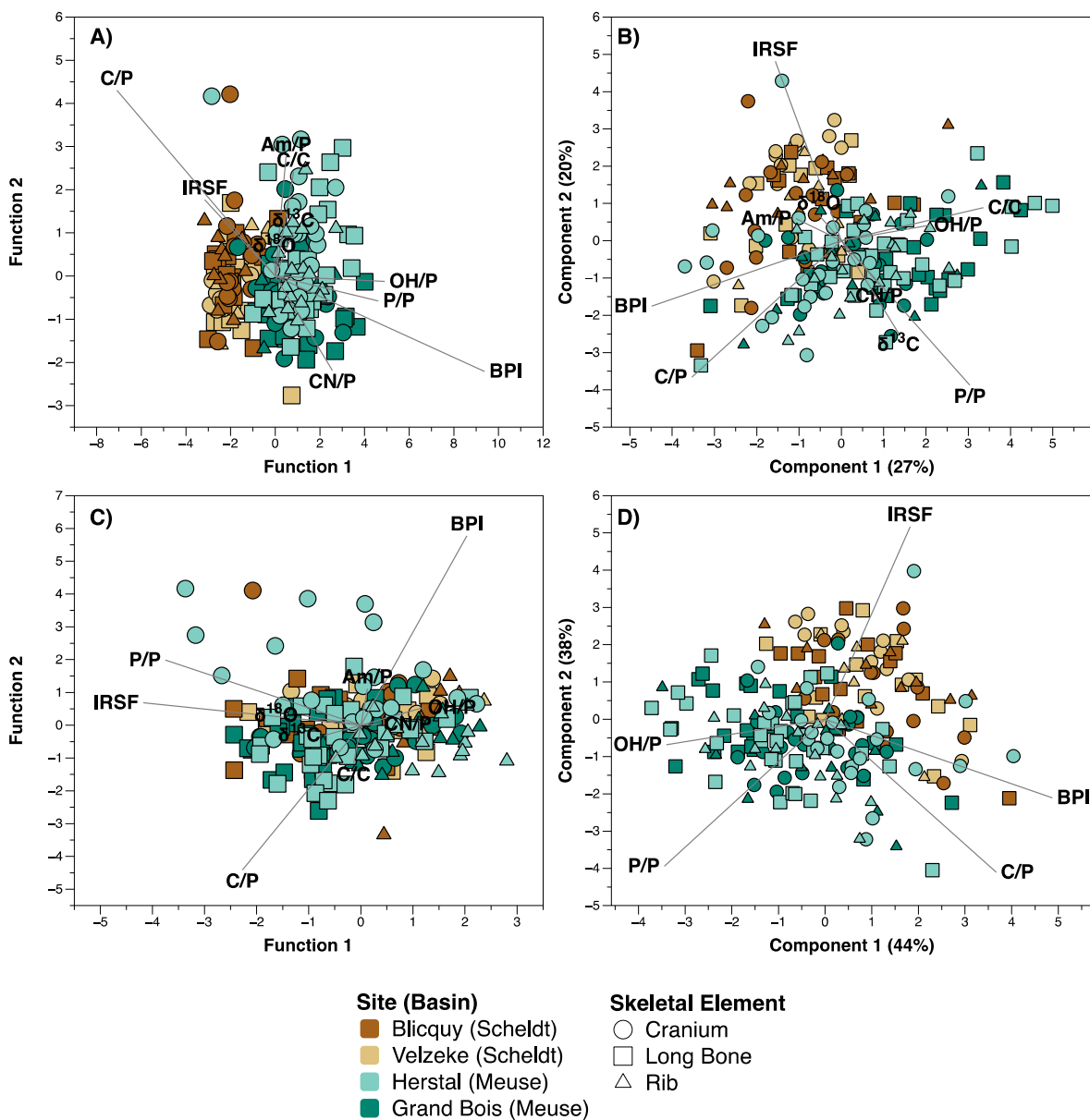
Fig. 4. Linear discriminant analysis (LDA) and principal components analysis (PCA) results. Marker fill colours indicate site of origin, and marker shapes indicate bone elements. Gray vectors indicate weightings of variables in each model. Panel A: LDA among Velzeke, Blicquy, Grand Bois and Herstal using all available variables; Panel B: PCA among Velzeke, Blicquy, Grand Bois and Herstal using all available variables; Panel C: LDA among bone elements using all available variables; Panel D: PCA among Velzeke, Blicquy, Grand Bois and Herstal using a reduced set of infrared variables (BPI, C/P, OH/P, P/P, and IRSF). (For interpretation of the references to colour in this figure legend, the reader is referred to the Web version of this article.)
