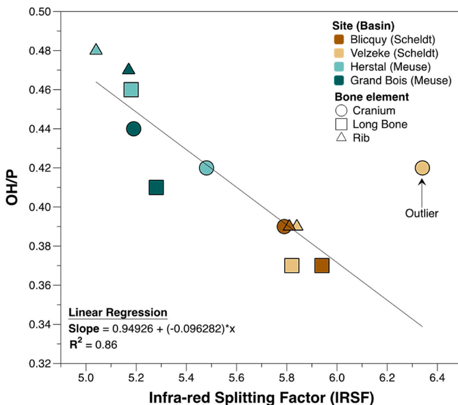
Fig. 5. Median values of OH/P to IRSF for the different skeletal element categories of the studied sites.
