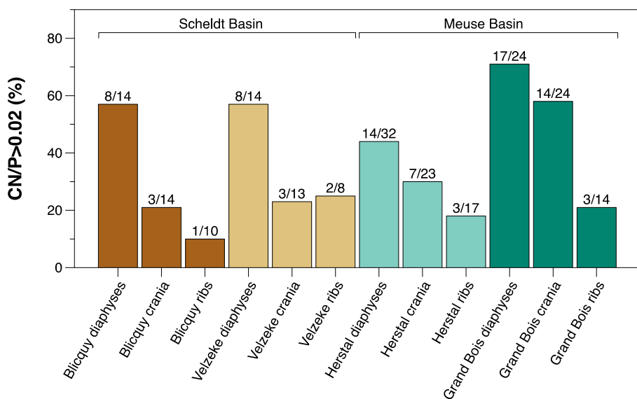
Fig. 6. Percentages samples with CN/P > 0.02 for the different skeletal element categories from Velzeke, Blicquy, Grand Bois and Herstal.
