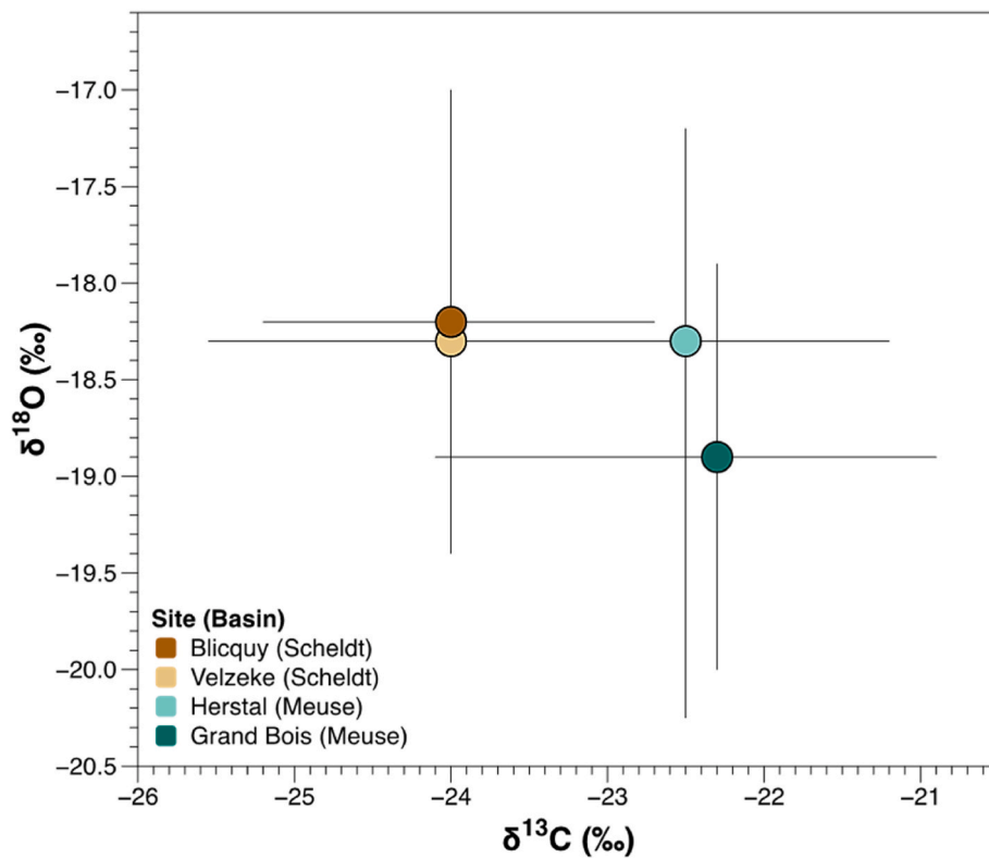
Fig. 2. Median \delta^{18}\text{O} to \delta^{13}\text{C} values of the studied sites. The error bars indicate the 1st and the 3rd quartiles.
