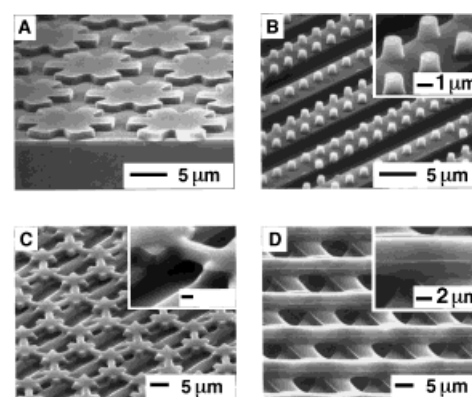
Figure 24. SEM images of polymeric microstructures fabricated by \mu\text{TM} : [36] A) patterned, isolated microstructures of PU on silver (one layer); B) isolated microcylinders of epoxy on 5- \mu\text{m} lines of epoxy supported on a glass slide (two layers); C) a continuous web of epoxy over a layer of 5- \mu\text{m} lines of epoxy supported on a glass slide (two layers); D) a three-layer structures on a glass slide made from a thermally curable epoxy.
