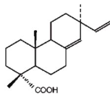
pimaric acid
