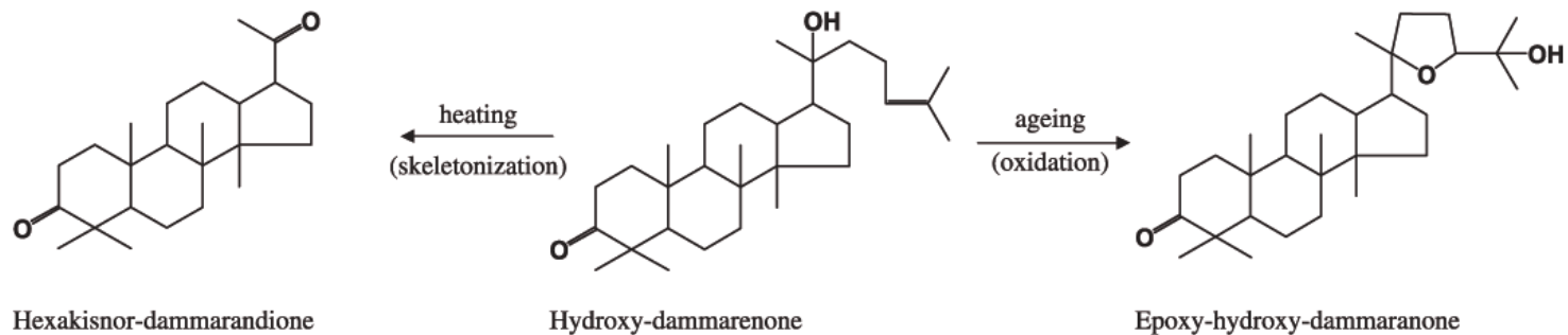
Scheme 1 Hydroxy-dammarenone and its ageing and heating products.
