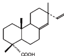
sandaracopimaric acid
