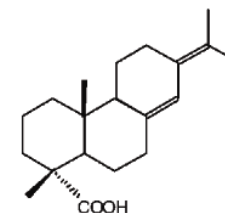
neoabietic acid
