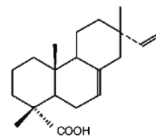
isopimaric acid
