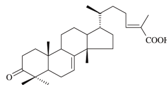
(iso)masticdienonic acid
