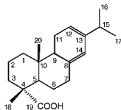
laevopimaric acid
