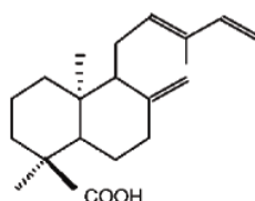
communic acid
