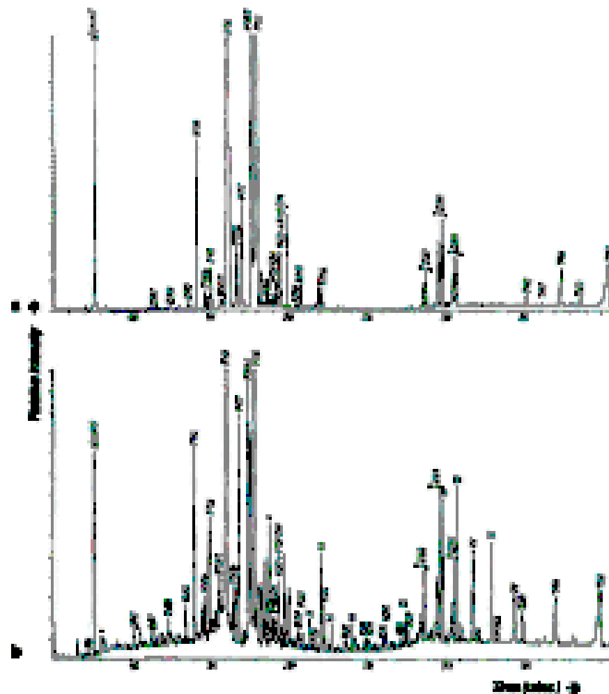
FIG. 4 Gas chromatograms showing the results from samples 85, 93 (a) and 93, 102 (b). All peaks are identified over the whole range from 10 to 100 minutes and carbon numbers. Peak identities were established by GC-MS. (a) Data — Decarboxylated acid with a carbon atom; C17 — Saturated fatty acid with a carbon atom; C18 — Decarboxylated fatty acid with a carbon atom; C19 — Mono-substituted fatty acid with a carbon atom; C20 — Hydroxy fatty acid with a carbon atom; C21 — Mono-substituted fatty acid with a fatty acyl carbon atom; C22 — Diacylfatty acid with a fatty acyl carbon; C23 — Diacylfatty acid with a fatty acyl carbon atom. Note that the diacylfatty acids correlate to C23 (not shown), C27, C31Ac — Diacylfatty acid with a carbon atom; C24 — Saturated fatty acid with a carbon atom; C25 — Saturated fatty acid with a carbon atom; C26 — Mono-substituted fatty acid with a carbon atom; C27 — Hydroxy fatty acid with a carbon atom; C28 — Mono-substituted fatty acid with a fatty acyl carbon atom; C29 — Saturated fatty acid with a carbon atom; C30 — Diacylfatty acid with a fatty acyl carbon atom; C31 — Saturated fatty acid with a carbon atom; C32 — Diacylfatty acid with a fatty acyl carbon atom; C33 — Saturated fatty acid with a carbon atom; C34 — Saturated fatty acid with a carbon atom; C35 — Saturated fatty acid with a carbon atom; C36 — Saturated fatty acid with a carbon atom; C37 — Saturated fatty acid with a carbon atom; C38 — Saturated fatty acid with a carbon atom; C39 — Saturated fatty acid with a carbon atom; C40 — Saturated fatty acid with a carbon atom; C41 — Saturated fatty acid with a carbon atom; C42 — Saturated fatty acid with a carbon atom; C43 — Saturated fatty acid with a carbon atom; C44 — Saturated fatty acid with a carbon atom; C45 — Saturated fatty acid with a carbon atom; C46 — Saturated fatty acid with a carbon atom; C47 — Saturated fatty acid with a carbon atom; C48 — Saturated fatty acid with a carbon atom; C49 — Saturated fatty acid with a carbon atom; C50 — Saturated fatty acid with a carbon atom; C51 — Saturated fatty acid with a carbon atom; C52 — Saturated fatty acid with a carbon atom; C53 — Saturated fatty acid with a carbon atom; C54 — Saturated fatty acid with a carbon atom; C55 — Saturated fatty acid with a carbon atom; C56 — Saturated fatty acid with a carbon atom; C57 — Saturated fatty acid with a carbon atom; C58 — Saturated fatty acid with a carbon atom; C59 — Saturated fatty acid with a carbon atom; C60 — Saturated fatty acid with a carbon atom; C61 — Saturated fatty acid with a carbon atom; C62 — Saturated fatty acid with a carbon atom; C63 — Saturated fatty acid with a carbon atom; C64 — Saturated fatty acid with a carbon atom; C65 — Saturated fatty acid with a carbon atom; C66 — Saturated fatty acid with a carbon atom; C67 — Saturated fatty acid with a carbon atom; C68 — Saturated fatty acid with a carbon atom; C69 — Saturated fatty acid with a carbon atom; C70 — Saturated fatty acid with a carbon atom; C71 — Saturated fatty acid with a carbon atom; C72 — Saturated fatty acid with a carbon atom; C73 — Saturated fatty acid with a carbon atom; C74 — Saturated fatty acid with a carbon atom; C75 — Saturated fatty acid with a carbon atom; C76 — Saturated fatty acid with a carbon atom; C77 — Saturated fatty acid with a carbon atom; C78 — Saturated fatty acid with a carbon atom; C79 — Saturated fatty acid with a carbon atom; C80 — Saturated fatty acid with a carbon atom; C81 — Saturated fatty acid with a carbon atom; C82 — Saturated fatty acid with a carbon atom; C83 — Saturated fatty acid with a carbon atom; C84 — Saturated fatty acid with a carbon atom; C85 — Saturated fatty acid with a carbon atom; C86 — Saturated fatty acid with a carbon atom; C87 — Saturated fatty acid with a carbon atom; C88 — Saturated fatty acid with a carbon atom; C89 — Saturated fatty acid with a carbon atom; C90 — Saturated fatty acid with a carbon atom. Note that the diacylfatty acids correlate to C23 (not shown).
