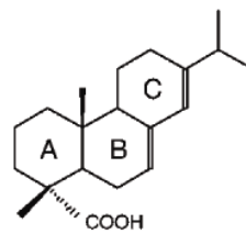
abietic acid
