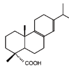
palustric acid
