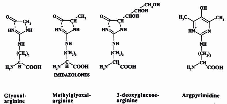
Fig. 8. Reactions of glucose and its metabolites, glyoxal, methylglyoxal and 3-deoxyglucosone with (a) lysine and (b) arginine in the formation of non-cross-linking AGEs. The consequent alteration of the charge profile of the collagen and elastin molecules leads to changes in the cell-matrix interactions.
