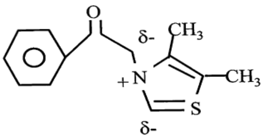
Fig. 1. The structure of N-phenacyl-4,5-dimethylthiazolium bromide (DMPTB).
