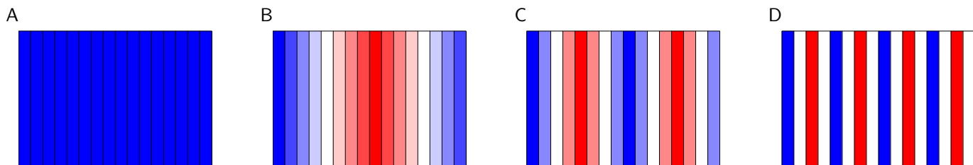
Figure 5.3: Phase-modulated pulses. A radio wave irradiation is divided into 16 pulses of different phases, distinguished by different colors. The blue and red colors correspond to 0^\circ and 180^\circ phases ( x and -x pulses), respectively, whereas white corresponds to 90^\circ and 270^\circ phases ( \pm y pulses). Magnetic moments irradiated by the pulses B, C, and D experience additional frequency of one, two, and four cycles per the pulse length, respectively. For example, if the pulse length is 100 \mu\text{s} , the pulses B, C, and D, respectively, resonate with the frequency higher by 10 kHz, 20 kHz, and 40 kHz than the carrier frequency.
