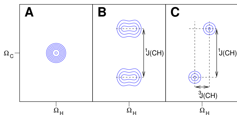
Figure 8.9: Peaks in a slice cut at the ^{15}\text{N} frequency from a conventional decoupled HNCA spectrum (A), coupled HNCA spectrum (B), and HNCA- J spectrum (C). The small ( < 10 Hz) three-bond coupling ^3J(\text{H}^{\text{N}}\text{H}^\alpha) is poorly resolved in the coupled HNCA spectrum, but well resolved in the HNCA- J spectrum due to the large (140 Hz) ^1J(\text{C}^\alpha\text{H}^\alpha) coupling.
