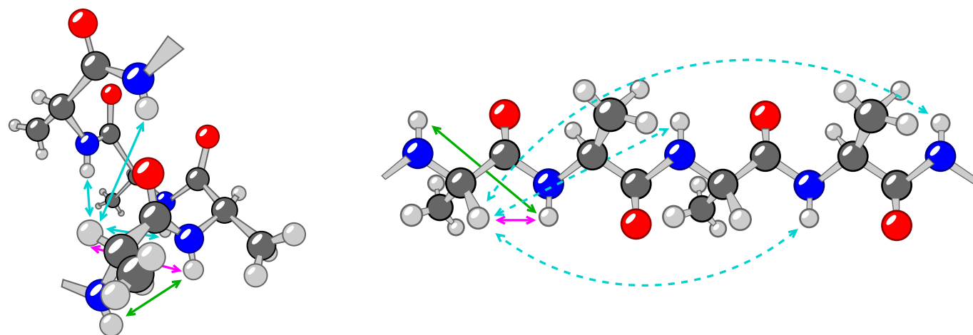
Figure 8.11: Proton-proton distances distinguishing \alpha -helix (left) from \beta -sheet (right). The distance between H_k^\alpha and H_{k+1}^N is shown in magenta, the distance between H_k^N and H_{k+1}^N is shown in green and the distances between H_k^\alpha and H_{k+2}^N , H_k^\alpha and H_{k+3}^N , H_k^\alpha and H_{k+4}^N are shown in cyan. Hydrogen, carbon, nitrogen, and oxygen atoms are shown in white, black, blue, and red, respectively.
