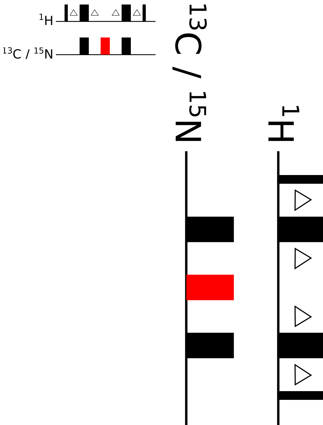
Figure 12.5: Isotope filter/edit pulse sequence element. The narrow and wide boxes represent the 90^\circ and 180^\circ pulse, respectively. All pulses are applied with the x -phase. Delays \Delta stand for 1/(4J) , where J is the J -coupling constant. The red pulse applied to ^{13}\text{C} / ^{15}\text{N} nucleus is either present (left) or omitted (right). Isotope-filtered and isotope-edited signals are obtained by adding and subtracting the spectra obtained using the individual elements, respectively.
