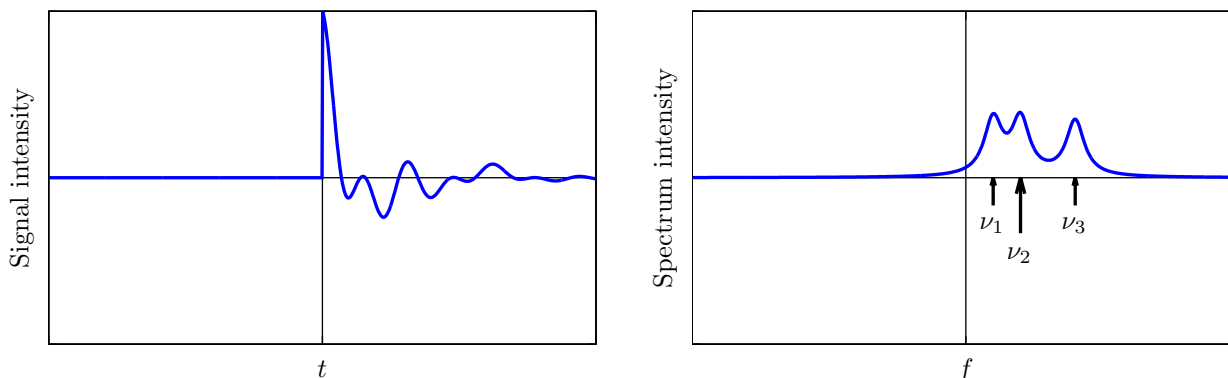
Figure 3.4: Signal (left) and frequency spectrum (right) with three precession frequencies.
