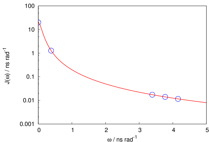
Figure 11.1: Example of the spectral density function with highlighted values of the spectral density values at frequencies that contribute to the relaxation rates of the ^{15}\text{N} - ^1\text{H} pair at 14.1 T (600 MHz spectrometer).
