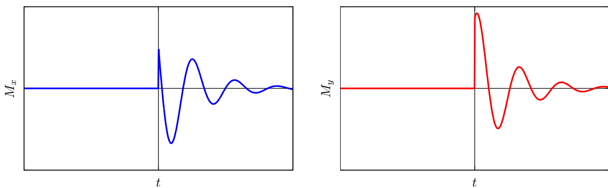
Figure 2.5: Values of M_x (blue) and M_y (red) components of a magnetization vector rotating with the initial phase of 60^\circ . The values decay due to a loss of coherence.
