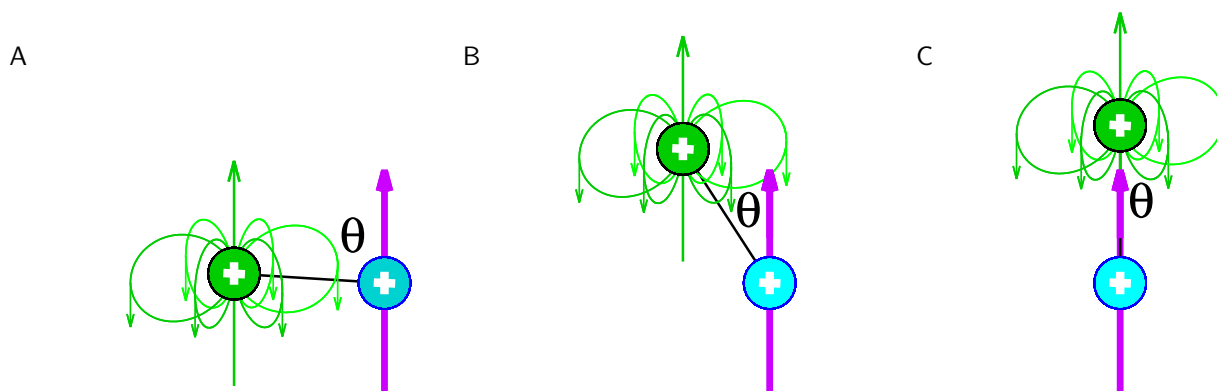
Figure 2.6: A, Classical description of interaction of a spin magnetic moment of the observed nucleus (shown in cyan) with a spin magnetic moment of another nucleus (shown in green). The thick purple arrow represents \vec{B}_0 , the thin green induction lines represent the magnetic field \vec{B}_2 of the green nucleus (the small green arrows indicate its direction). The black line represents the internuclear vector \vec{r} . As the molecule rotates, the cyan nucleus moves from a position where the field of the spin magnetic moment of the green nucleus \vec{B}_2 has the opposite direction than \vec{B}_0 (A), through a position where \vec{B}_2 is perpendicular to \vec{B}_0 (B), to the position where \vec{B}_2 has the same direction as \vec{B}_0 (C).
