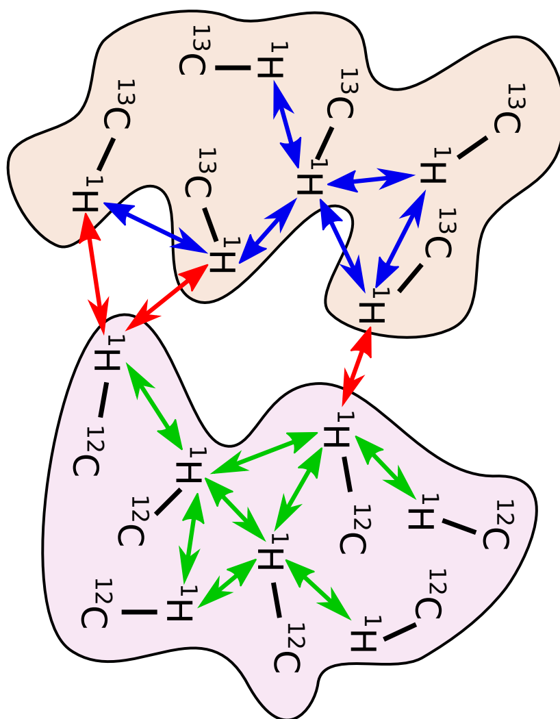
Figure 12.6: Contacts detected by the isotope filtered/edited NOE experiment. The light yellow molecule was prepared with ^{13}\text{C} isotope enrichment, unlike the light magenta molecule. The blue arrows mark intramolecular contacts within the ^{13}\text{C} labeled molecule that can be selectively detected by inserting the isotope editing element before and after the NOE mixing time. The green arrows mark intramolecular contacts within the ^{13}\text{C} unlabeled molecule and can be selectively detected by inserting the isotope filtering element before and after the NOE mixing time. The red arrows show inter-molecular NOE contacts selectively detected if the isotope filtering element is placed before the NOE mixing time and the isotope editing element is placed after it, or vice versa.
