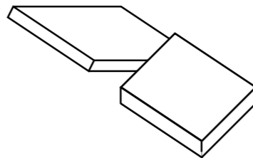
Propeller twist ( \omega )
