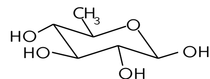
D-chinovopyranosa- ^4C_1
