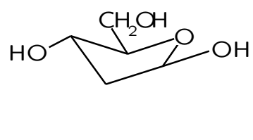
2-deoxy-D-ribose- ^3E
