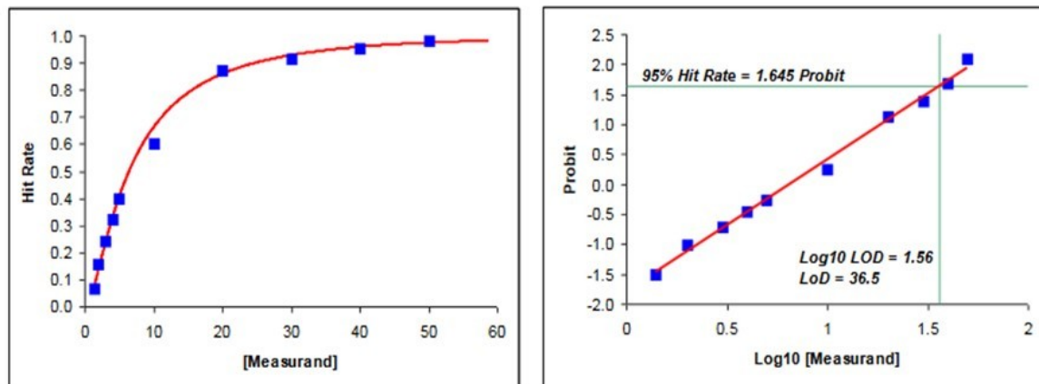
Figure 3. Probit Analysis. These plots illustrate hypothetical experimental results (left hand plot) an regression analysis to determine the LoD for a molecular measurement procedure by the probit approach (right hand plot).
