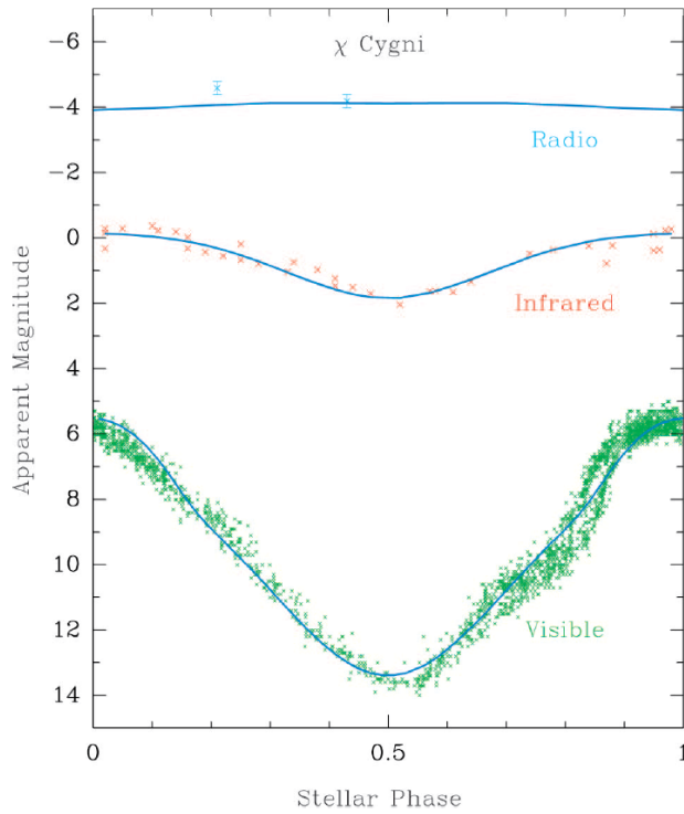
FIG. 4.—Observed radio (cyan), infrared (red), and visible (green) light curves for the Mira variable \chi Cygni. (See text for references.) Solid blue lines are from a simple model of an oxygen-rich Mira variable with an extended atmosphere. Near stellar phase of 0.5, molecular absorption, mostly by TiO, enlarges the apparent visible size of the star to nearly 2R_* . The low atmospheric temperatures ( \approx 1400 K) at this radius result in an \approx 8 mag decrease in visible light compared to maximum light. The infrared data are insensitive to molecular absorption and respond mostly to the central pulsating star. The radio emission is sensitive to the free electron density, and high radio opacity, owing to H^- free-free interactions, occurs near \approx 2R_* throughout the stellar cycle.
