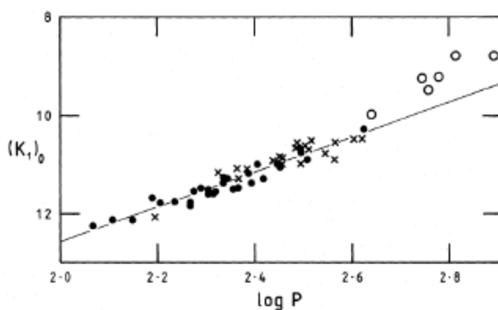
Figure 2.5: A K - \log P -diagram for detected Mira variables in the LMC taken from Feast et al. (1989). Filled circles denote O-rich Miras with periods < 420 d, open circles O-rich Miras with periods > 420 d and crosses C-rich Miras.
