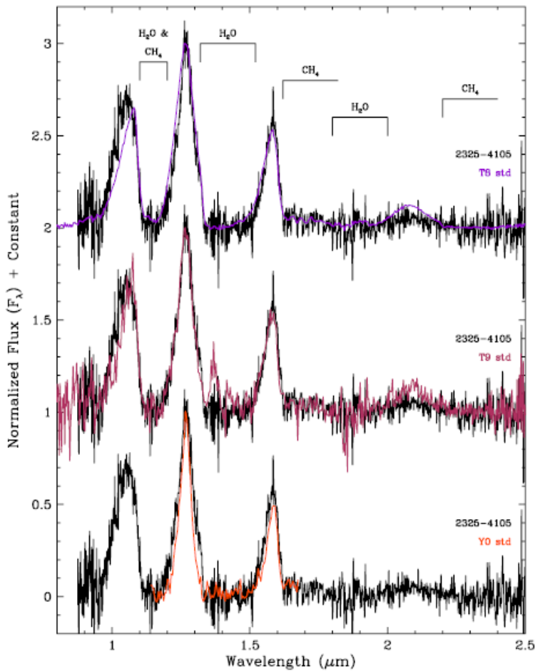
Figure 44. Near-infrared spectrum of WISE 2325–4105 (black) compared to the T8 (dark violet), T9 (maroon), and Y0 (orange red) spectral standards from Burgasser et al. (2006b) and Cushing et al. (2011). Spectra have been normalized to one at 1.28 \mu\text{m} and integral offsets have been added to the y-axis values to separate the spectra vertically except where overplotting was intended. Prominent spectral features are marked.
