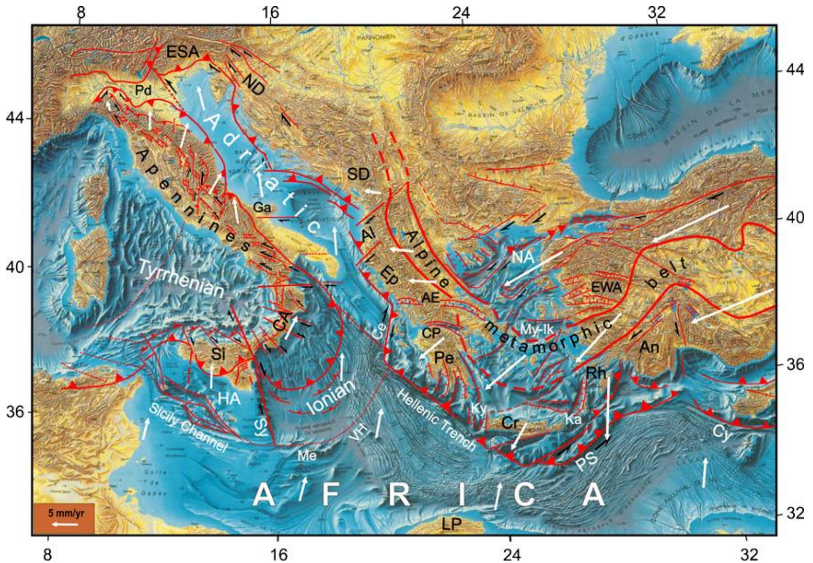
(Viti et al. 2010)
