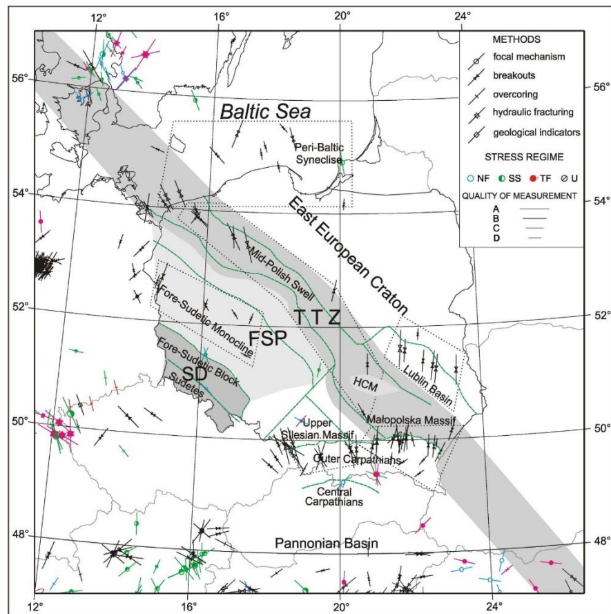
Fig. 1. Intraplate stress indicators showing the maximum horizontal stress ( S_{1max} ) directions for Poland and adjacent areas from the World Stress Map Database (Reinecker et al. , 2005), supplemented with data provided by Wiejacz (1994, 2004), Dębski et al. (1997), Roth and Fleckenstein (2001), Jarosiński (2005a)
