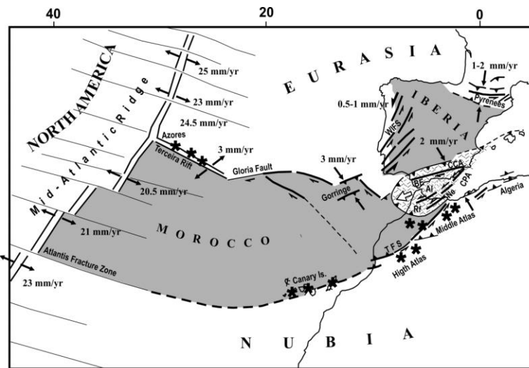
(Mantovani et al. 2007)
