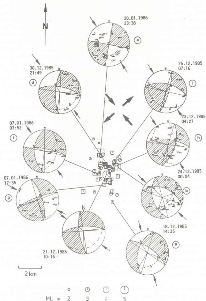
Fig. 8. Focal mechanisms and spatial distribution of foci for the 1985/86 Western Bohemia earthquake sequence. The balloon diagrams are keyed to Fig. 7. Octagons and squares are epicenters located during the period Dec. 18, 1985 to Feb. 6, 1986. Reverse oblique-slip faulting ((h), (i), (g)) occurs south-west and north-east of the December main shock. The mechanisms (e), (d), (f), the main shock (h), and (a), situated from north to south along the Mariánské Lázně Fault, indicate an increasing normal faulting component to the south of the active area. The direction of the P-axes of the fault plane solutions and the average orientation of the horizontal local stress field are also indicated.
