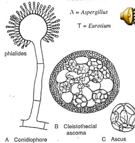
4.7 Eurotialean holomorph.
