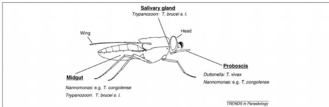
Figure 1. Development sites of trypanosomes of medical and veterinary importance in tsetse flies. When trypanosomes are found in the proboscis only, they are designated as belonging to subgenus Duttonella ( T. vivax ). When they are found in the proboscis and midgut, they are listed in the subgenus Nannomonas (e.g. T. congolense ), and when they are found in the midgut, proboscis and salivary glands, they are designated to the subgenus Trypanozoon ( T. brucei group). When trypanosomes are only found in the midgut, they are said to be immature and not classified.
