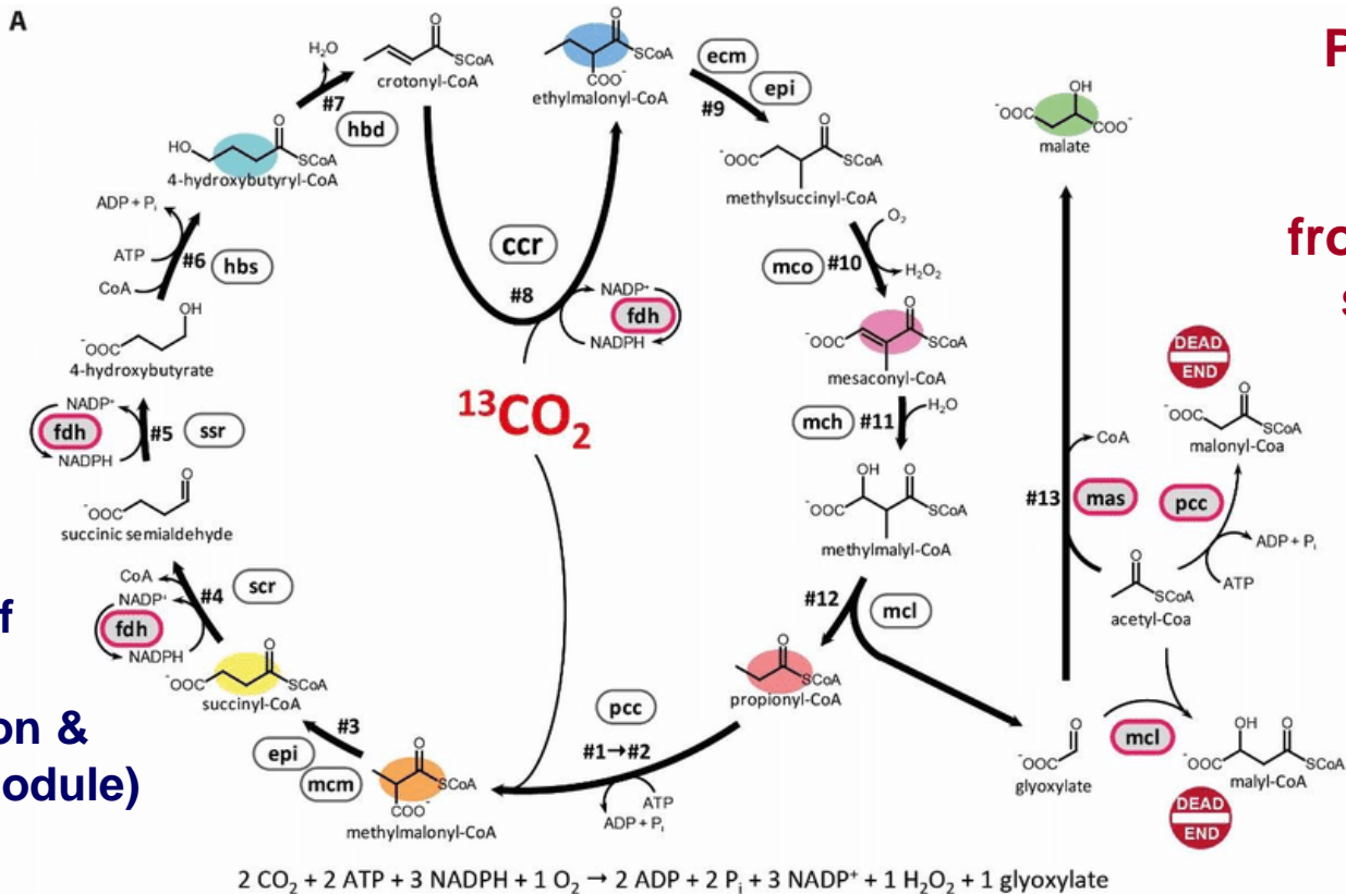
(A) Topology of the CETCH cycle version 3.0. The newly added enzymes Fdh (NADPH regeneration) and Mas (read-out module) converting the primary CO 2 -fixation product glyoxylate into malate are boxed in red.
