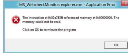
Segmentation Fault
