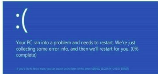
Kernel Fault
