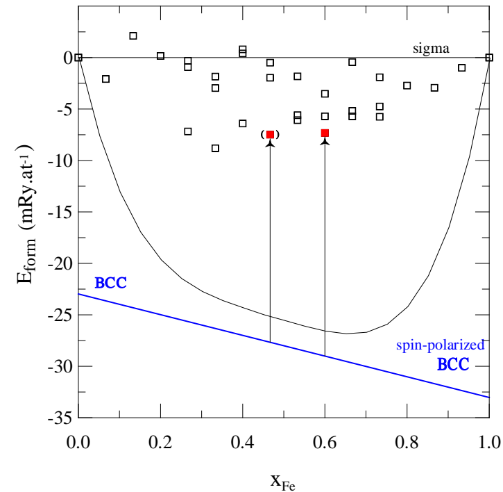
Fig. 2a. CrFe system: Enthalpy of formation of sigma phase with respect to SER standard state.
