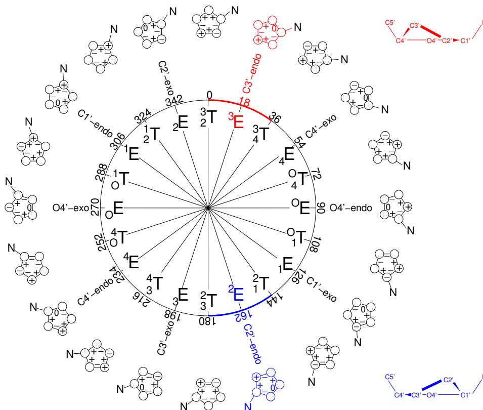
Figure 13.4: Values of P displayed using the pseudorotation wheel . All envelope and twisted conformations are marked (starting from the center by one-letter symbol, value of P , verbal description, and depicted schematically (circles symbolize atoms in the furanose ring, plus and minus signs mark atoms in the endo and exo positions, respectively, and signs of the angles \nu_i are displayed next to the bonds). Conformations C2' -endo- and C3' -endo are shown in blue and red, respectively).
