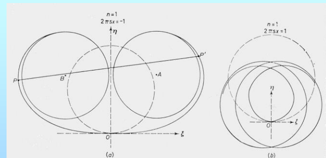
Amplitude-phase diagrams for a column of crystal close to a screw dislocation (Figure 7.13). (a) n=1, 2\pi s x = -1 ; (b) n=1, 2\pi s x = +1 . The amplitude diffracted by column EF in Figure 7.13 is given by the line joining points P and P' corresponding to the top and bottom of the crystal. The separation between P and P' measured along the curves is equal to the crystal thickness. The amplitude diffracted from one side of the dislocation (a) is greater than that from the other side (b).
