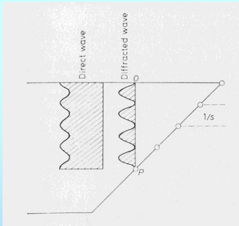
Figure 23.2. (A) At the Bragg condition ( s = 0 ), the intensities of the direct and diffracted beams oscillate in a complementary way. (B) For a wedge specimen, the separation of the fringes in the image (C) is determined by the angle of the wedge and the extinction distance, \xi_g .
