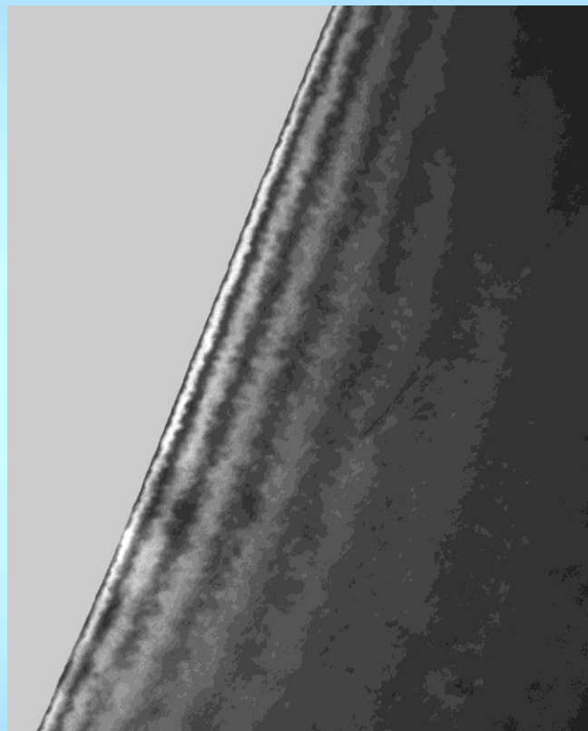
Figure 23.2. (A) At the Bragg condition ( s = 0 ), the intensities of the direct and diffracted beams oscillate in a complementary way. (B) For a wedge specimen, the separation of the fringes in the image (C) is determined by the angle of the wedge and the extinction distance, \xi_g .
