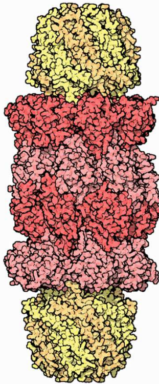
proteasom
