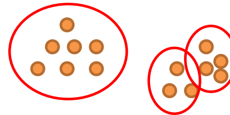
K-means k=3
