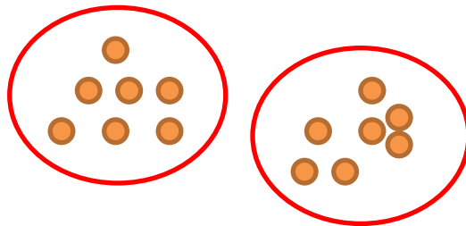
K-means k=2
